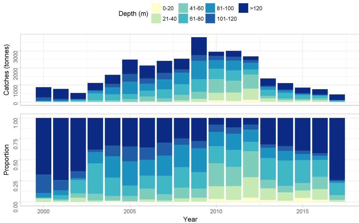
Figure3. Anglerfish. Depth distribution of catches according to logbooks.
