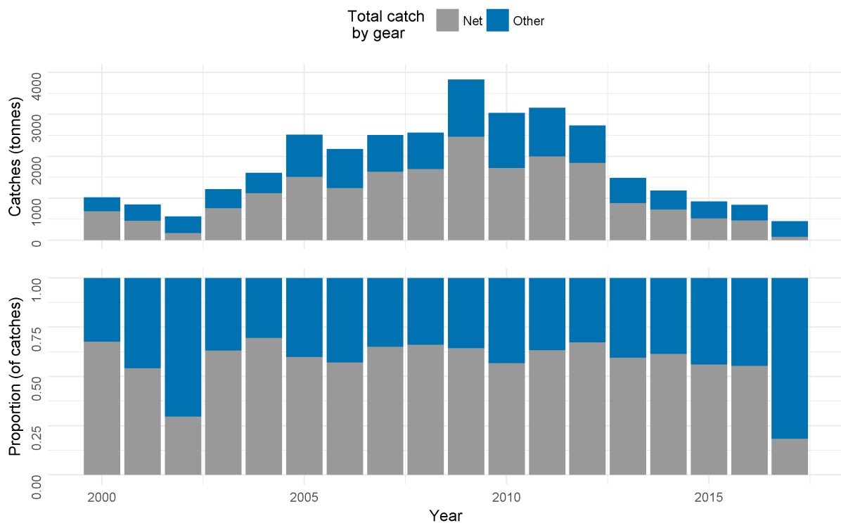
Figure 4. Anglerfish. Total catches and proportion captured with gillnets from 2000 to 2017 as reported in logbooks.
