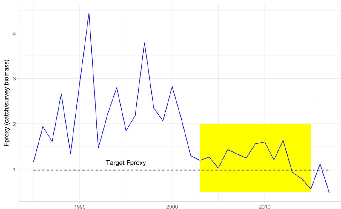
Figure 13. Anglerfish. F_{\text{proxy}} (catch/survey biomass). The target F_{\text{proxy}} is set as 80% of the mean value for the reference period (in yellow, 2003-2015).
