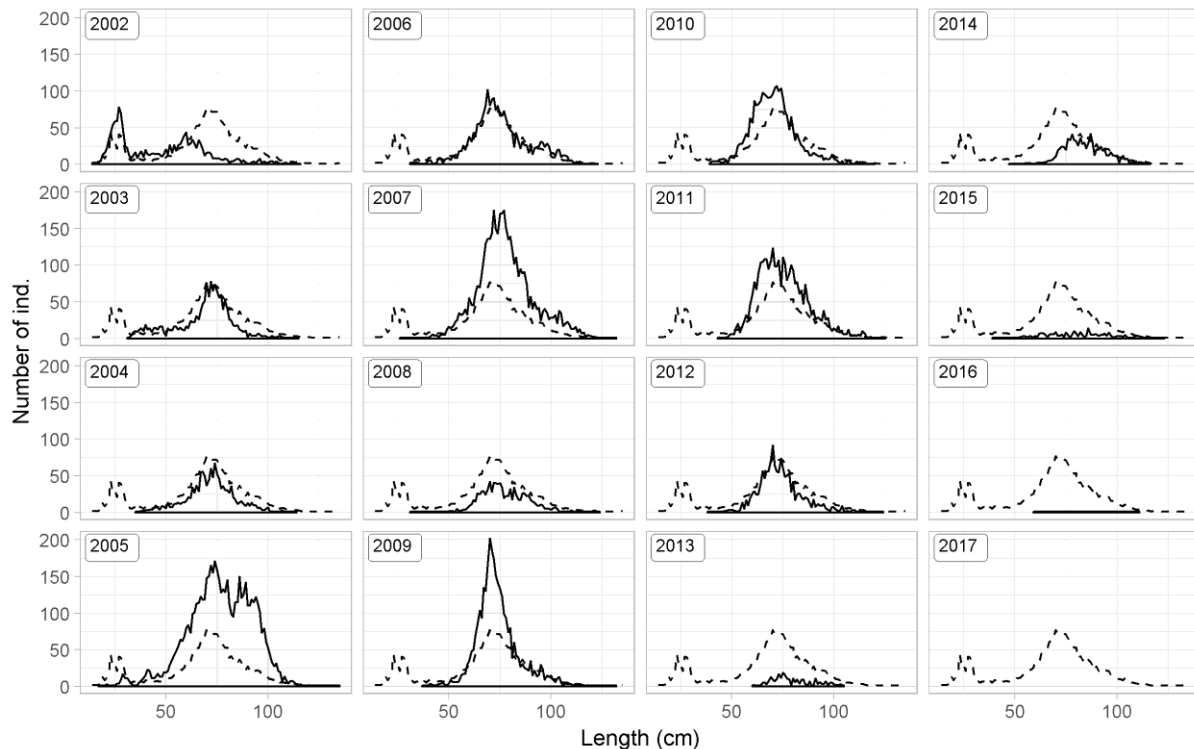
Figure 5. Anglerfish. Length distribution from commercial catches 2002-2017. Dotted lines indicate the average length distribution in 2002-2017.
