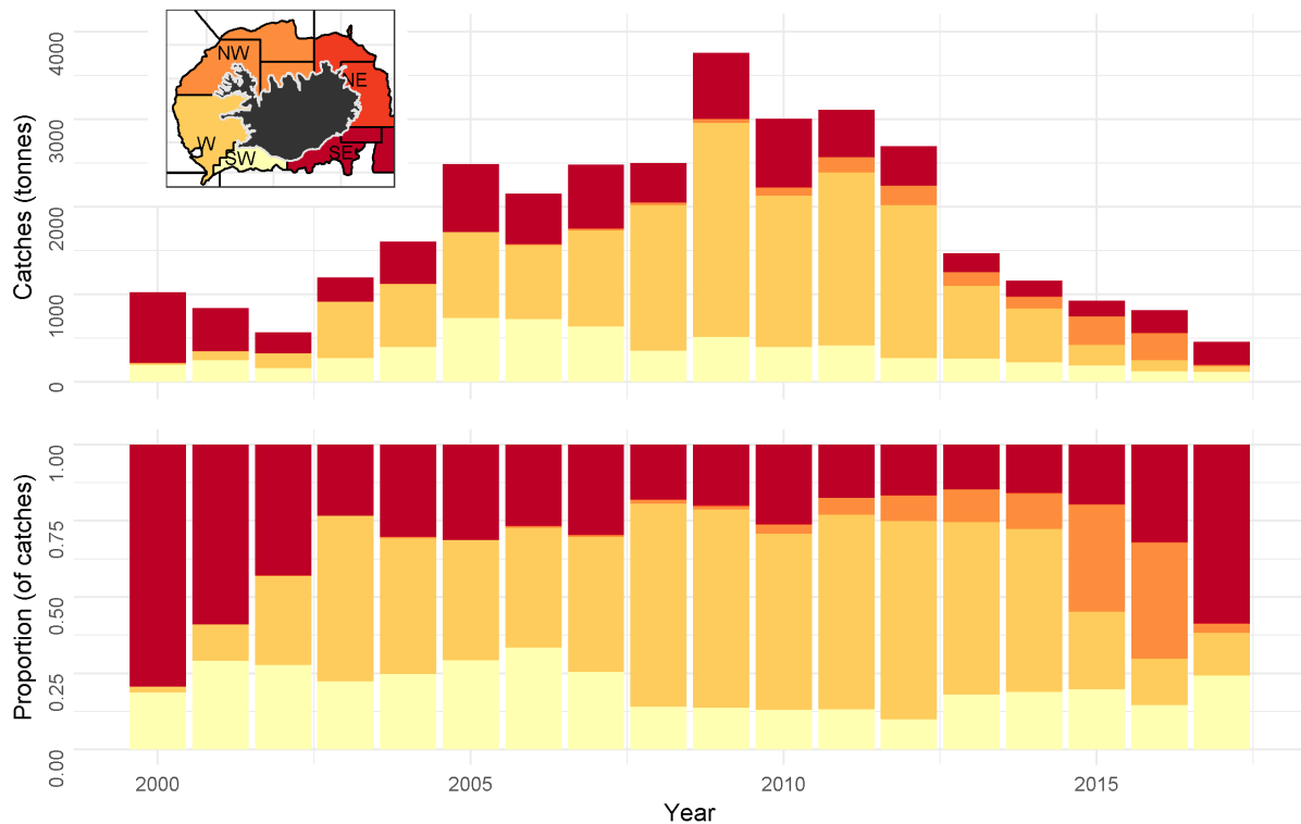
Figure 2. Anglerfish. Catch distribution and proportions by area from the year 2000 according to logbooks.
