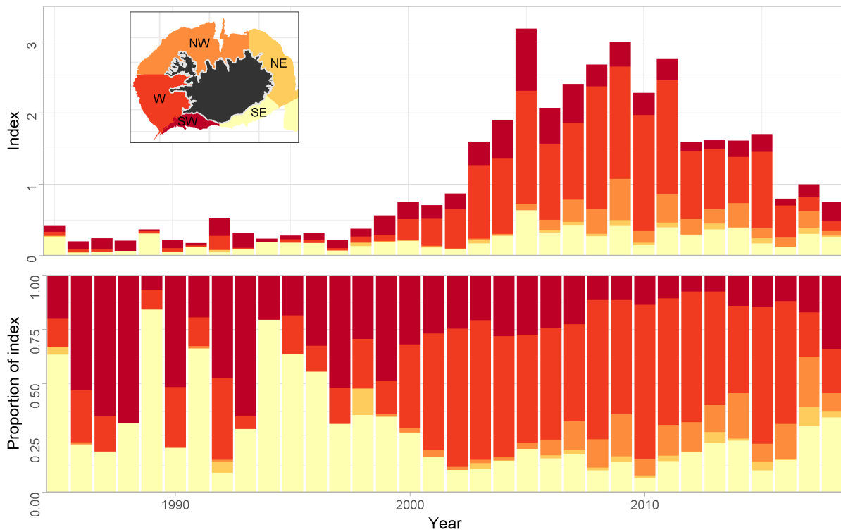
Figure 9. Anglerfish. Spatial distribution of catches from the spring groundfish survey in 1985-2017.
