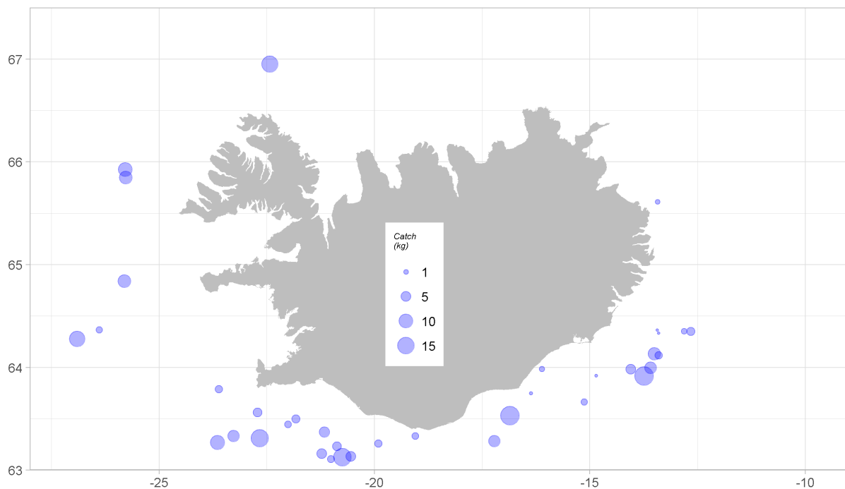
Figure 8. Anglerfish. Spatial distribution from the spring groundfish survey in 2018.
