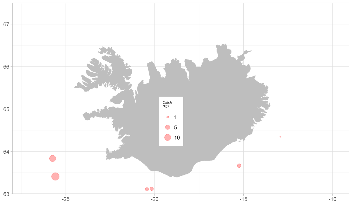
Figure 10. Anglerfish. Spatial distribution of catches from the autumn groundfish survey 2017.
