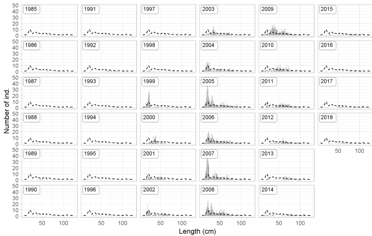
Figure 7. Anglerfish. Length distribution from the spring survey. The dotted line indicates mean length for all years.
