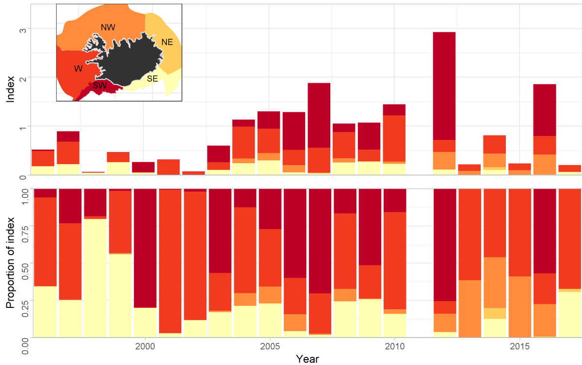
Figure 11. Anglerfish. Spatial distribution of catches from the autumn groundfish survey in 1996-2017.
