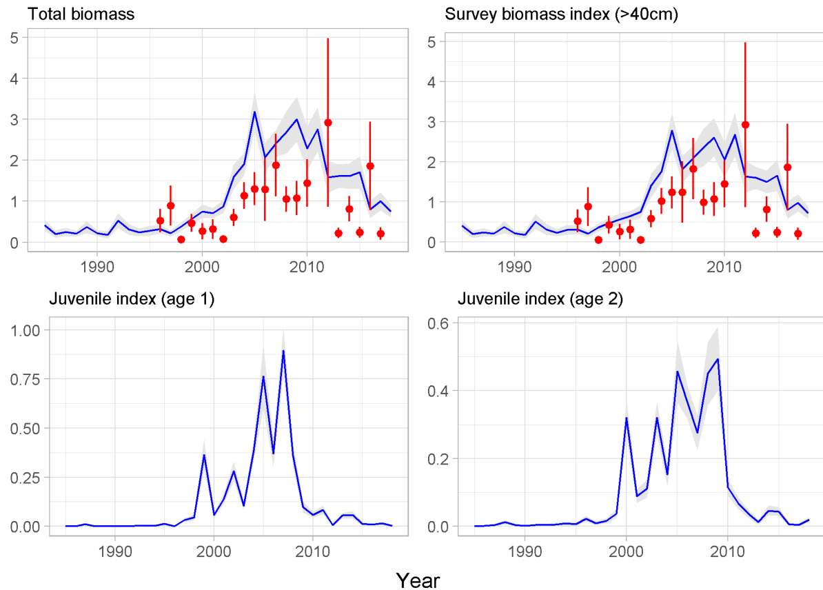
Figure 6. Anglerfish, Total groundfish survey biomass index, reference biomass index (>40cm) and juvenile indices for one and two year olds. Blue lines indicate spring survey and red dots indicate autumn survey. Shaded areas and error bars indicate coefficient of variance.
